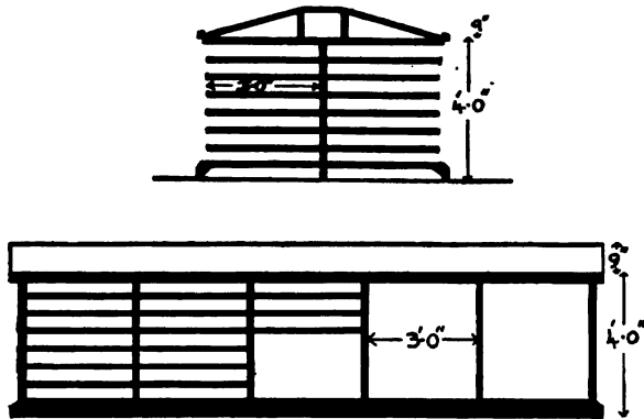
FIG. 44.—Section and Elevation of Case for Large Folio Books (Section 186).
